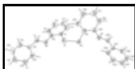
Fig. 1. The title molecule with the atomic numbering scheme. The displacement ellipsoids are shown at the 30% probability level.
